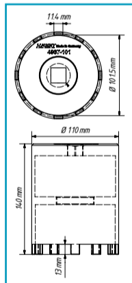
Slotted nut
