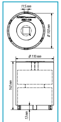
Slotted nut
