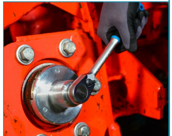
Operating using ratchet with inserted 12.5 mm (1/2") 4-point socket
