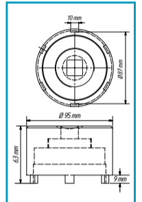
Slotted nut
