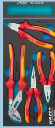
Pliers set · with protective insulation 163-226/4 ● 759N-2VDE · 1803VDE-22 · 1841BVDE-33 · 1850VDE-22
